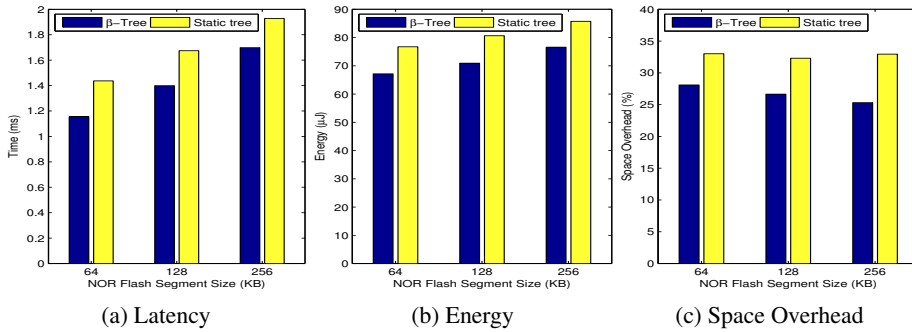
Fig. 2. Performance per insertion
